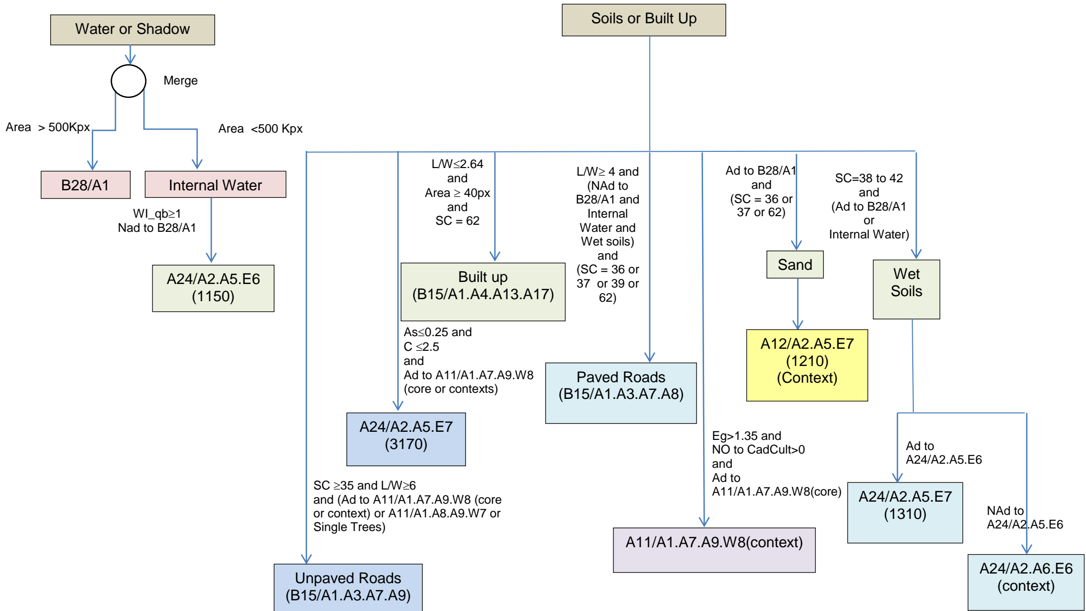
Figure F1.7 a) 2 nd stage hierarchical processing chain for Water or Shadow and Bare Soils or Built-up SIAM™ strata. At 2.4 m spatial resolution shadow is not detectable.
