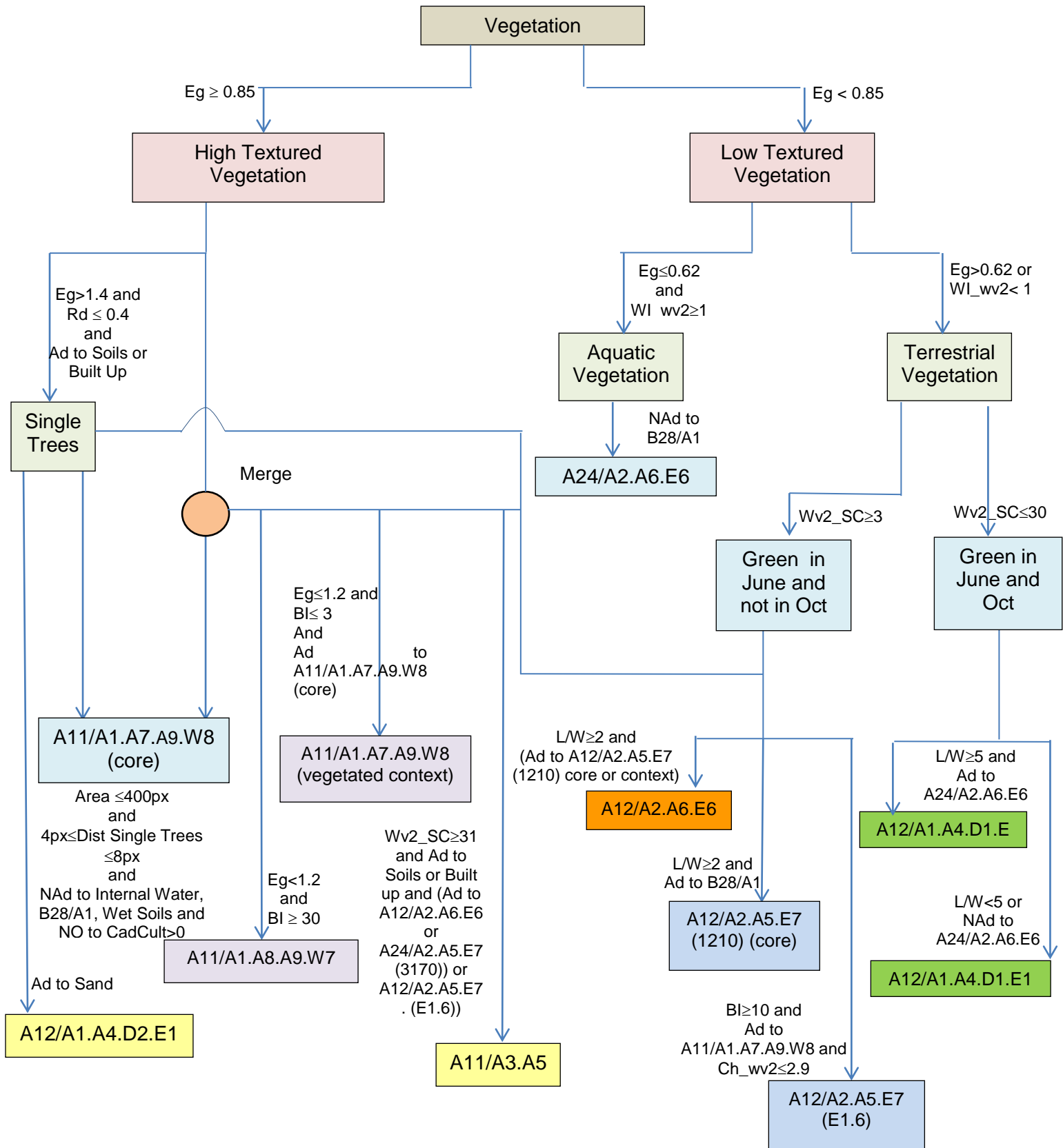
Figure F1.7 b) 2 nd stage hierarchical processing chain for Vegetation SIAM™ strata.
