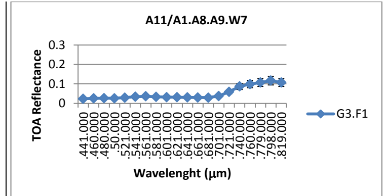
MIVIS VNIR Spectrum acquired on 24 th May 2009 (spatial resolution =3m)
