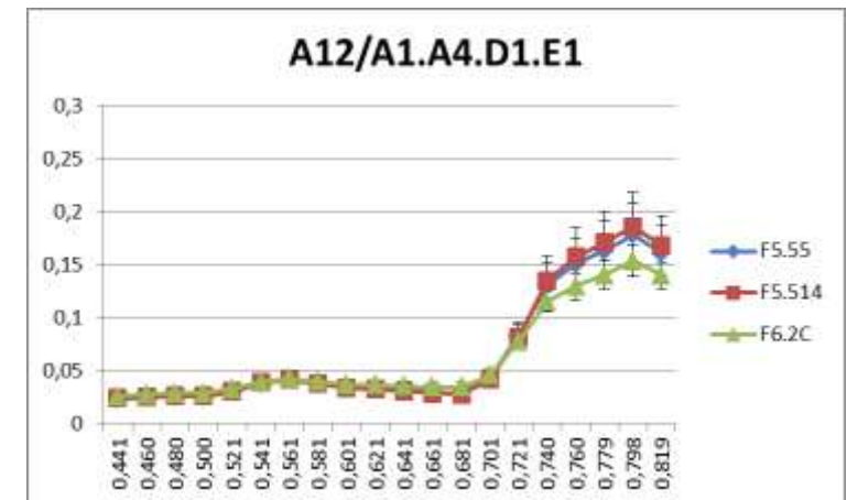
MIVIS VNIR Spectrum acquired on 24 th May 2009
