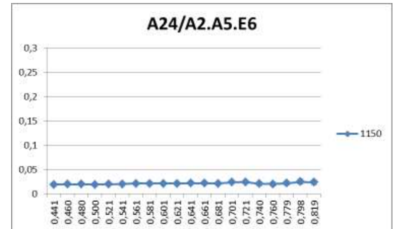
MIVIS VNIR Spectrum acquired on 24 th May 2009 (spatial resolution =3m)
