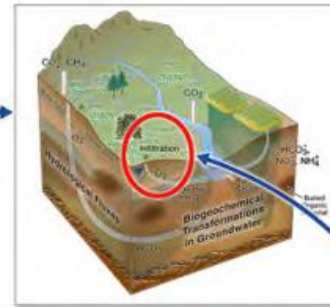
Catchment-scale hydro/biogeochem
