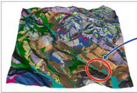
Watershed-scale processes
