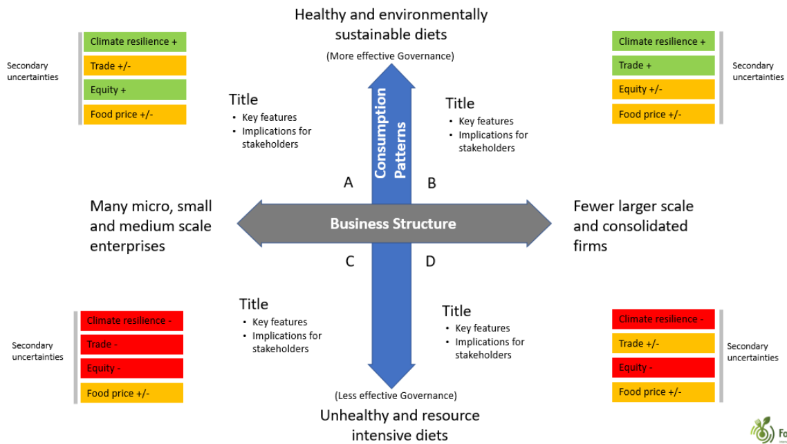
Figure 12 First scenario matrix based on two critical uncertainties
